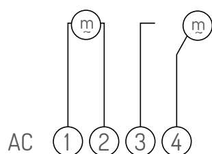
Ex9TAMS
