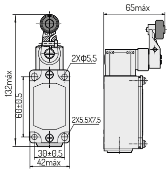
YBLX-P1/120/1G
