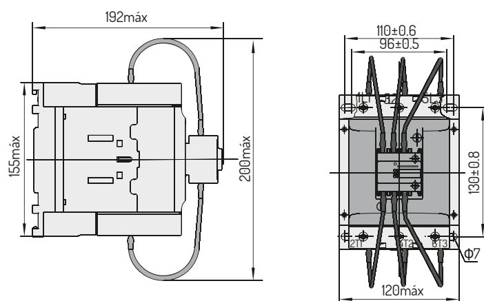
CJ19-115~170
