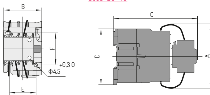
CJ19-25~43
