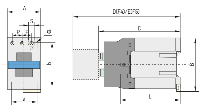
NC1-12Z~32Z
