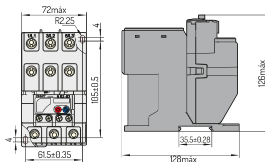
NR2-93 com MB-4
