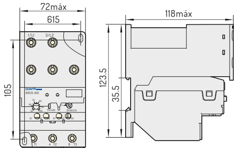
NRE8-100/F
