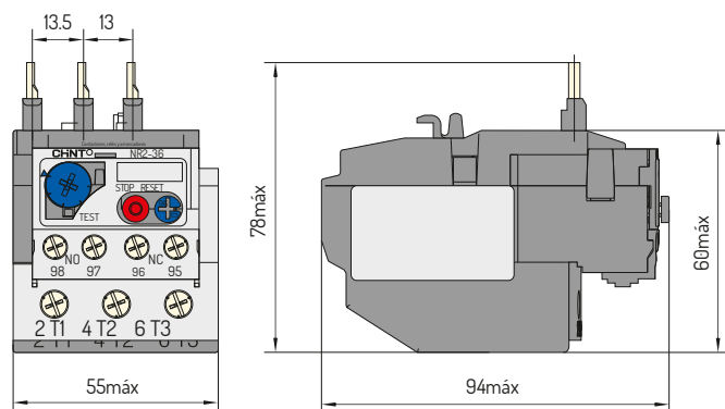
NR2-36
