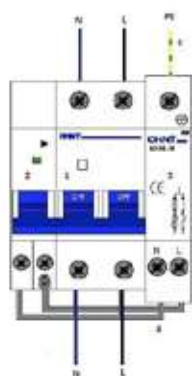
SOST2 (20-63)
