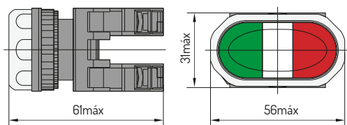
NP8-S
