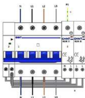
SOSTC4 (16-63A)
