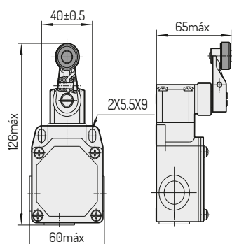
YBLX-P1/100/1G
