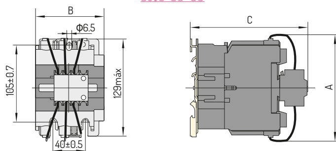
CJ19-63~95
