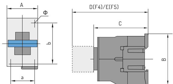
NC1-12~32
