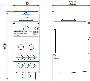
PDB 1P 1CU 1x6 160A
