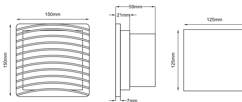
NTF1-045.230/NTF1-045.300
